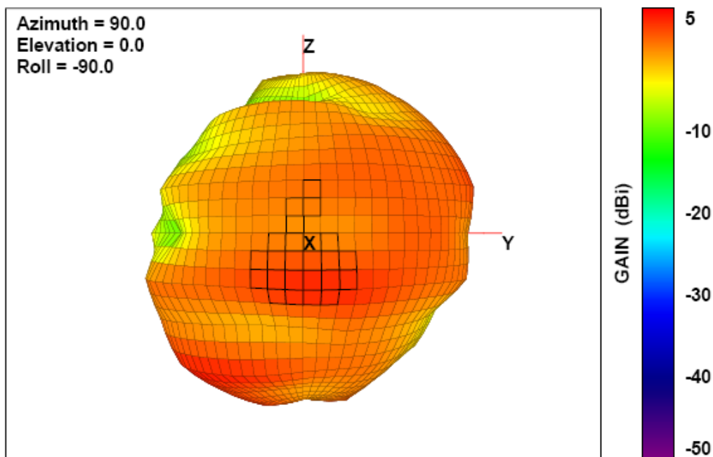
Free-Space Total GAIN, Left Side View, 2450.0 MHz
