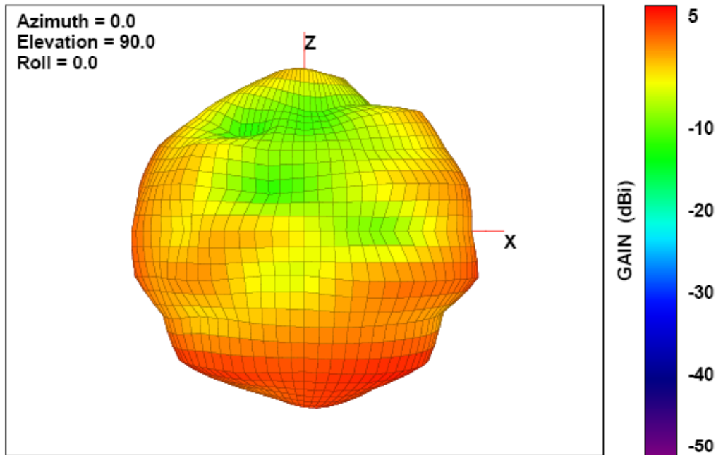
Free-Space Total GAIN, Back Face View, 2450.0 MHz
